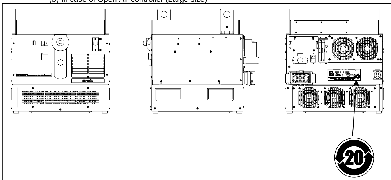
(b) In case of Open Air controller (Large size)
